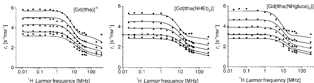
Fig. 4. NMRD Profiles of [\text{Gd}(\text{ttha})]^{3-} , [\text{Gd}(\text{ttha}(\text{NHET})_2)]^- , and [\text{Gd}(\text{ttha}(\text{NHgluca})_2)]^- with best fit curves (see text) at 5 (■), 15 (●), 25 (▲), 37 (▼), and 45° (◆)
